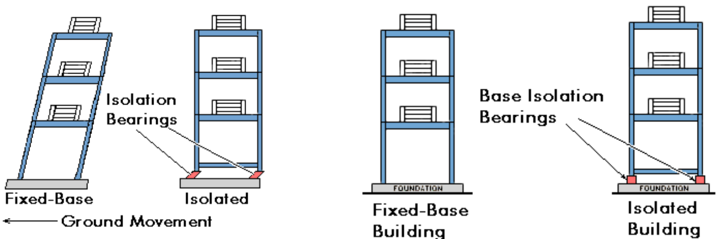
Movement of Building with Base Isolation vs. No Base Isolation
